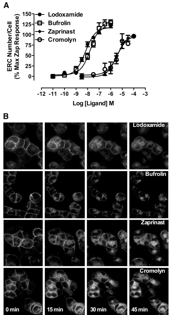
Fig. 3. High content analysis of internalization of human GPR35a confirms agonism of certain antiallergenics at this receptor. (A) The capacity of varying concentrations of lodoxamide (●), bufrolin (□), zaprinast (◆), or cromolyn disodium (○) to promote internalization of human GPR35a-eYFP was assayed and quantified via high content analysis as number of endocytic recycling compartments (ERCs) per cell. (B) Representative images of the cellular distribution of human FLAG-GPR35a-eYFP at the times indicated after addition of maximally effective concentrations of lodoxamide (5 \mu M), bufrolin (100 nM), zaprinast (50 \mu M), and cromolyn disodium (100 \mu M) are displayed.
