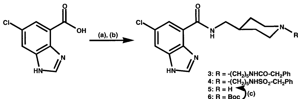
Scheme 1. Synthesis of 6-chlorobenzimidazole-4-carboxamides 3-6.
