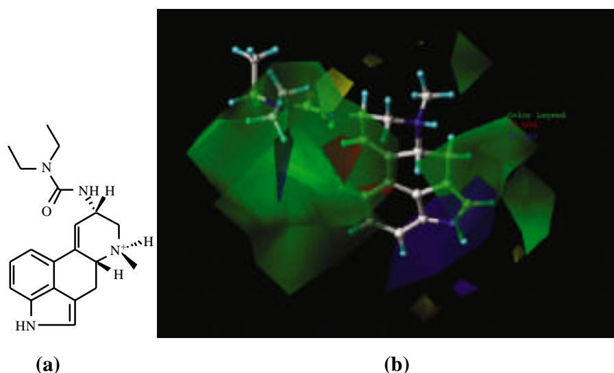
Fig. (5). (a) 2D structure of R -lisuride, compound used as template for the alignment of the molecules included in the CoMFA study. (b) Contour map relating compound affinity at 5-HT 7 R s to electrostatic and steric intermolecular interaction fields using lisuride. Positive electrostatic charge is favored (blue) or not favored (red) for high-affinity (80:20). Steric bulk is favored (green) or not favored (yellow) for high-affinity (80:20). See reference [75].
