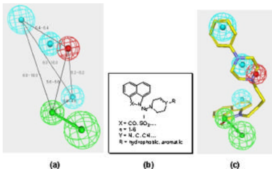
Fig. (6). (a) Pharmacophore model for selective 5-HT 7 R antagonists. (b) Designed naphtholactam and naphthosultam derivatives of general structure I. (c) Designed compound I (X = CO, n = 4, Y = N, R = phenyl) mapped on the hypothesis generated for 5-HT 7 R antagonists.
